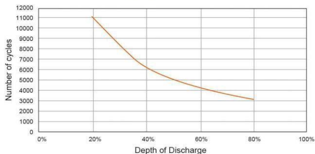
Battery cycle life vs DOD
